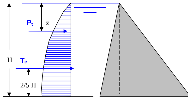
Figure 22 : Force hydrodynamique (Seghir, 1999)
