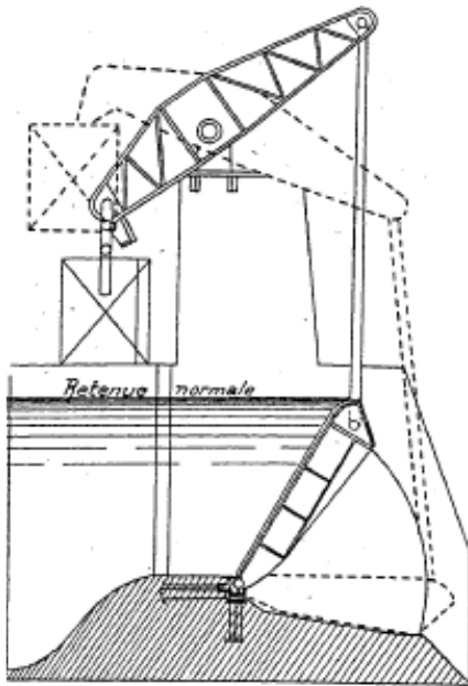
Figure 57 : Vanne Clapet
